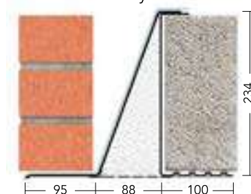
90-105mm cavity
